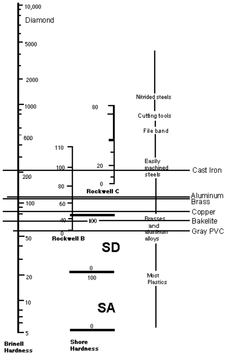
Aproximate Comparison of Hardness Scales
